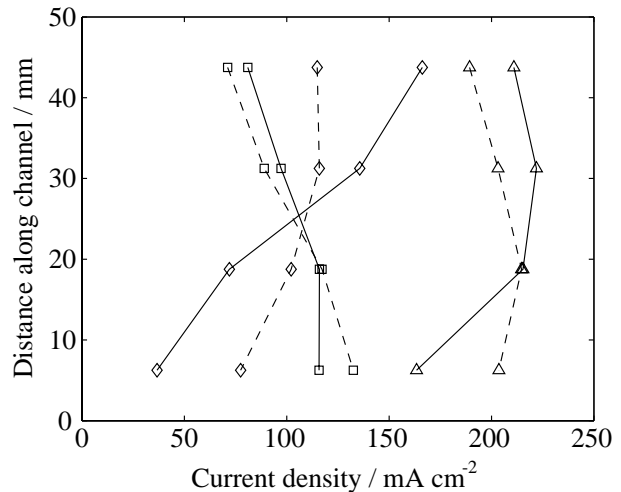
Fig. 8. Current distributions averaged in the horizontal direction. T_{\text{cell}} = 40\text{ }^{\circ}\text{C} , j_{\text{ave}} = 100\text{ mA cm}^{-2} ( \square ); T_{\text{cell}} = 60\text{ }^{\circ}\text{C} , j_{\text{ave}} = 100\text{ mA cm}^{-2} ( \diamond ); T_{\text{cell}} = 60\text{ }^{\circ}\text{C} , j_{\text{ave}} = 200\text{ mA cm}^{-2} ( \Delta ). Anode in dead-end mode, general directions of hydrogen flow down (---) and up (—).
